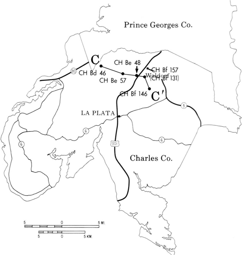
Location of Hydrogeologic Section
