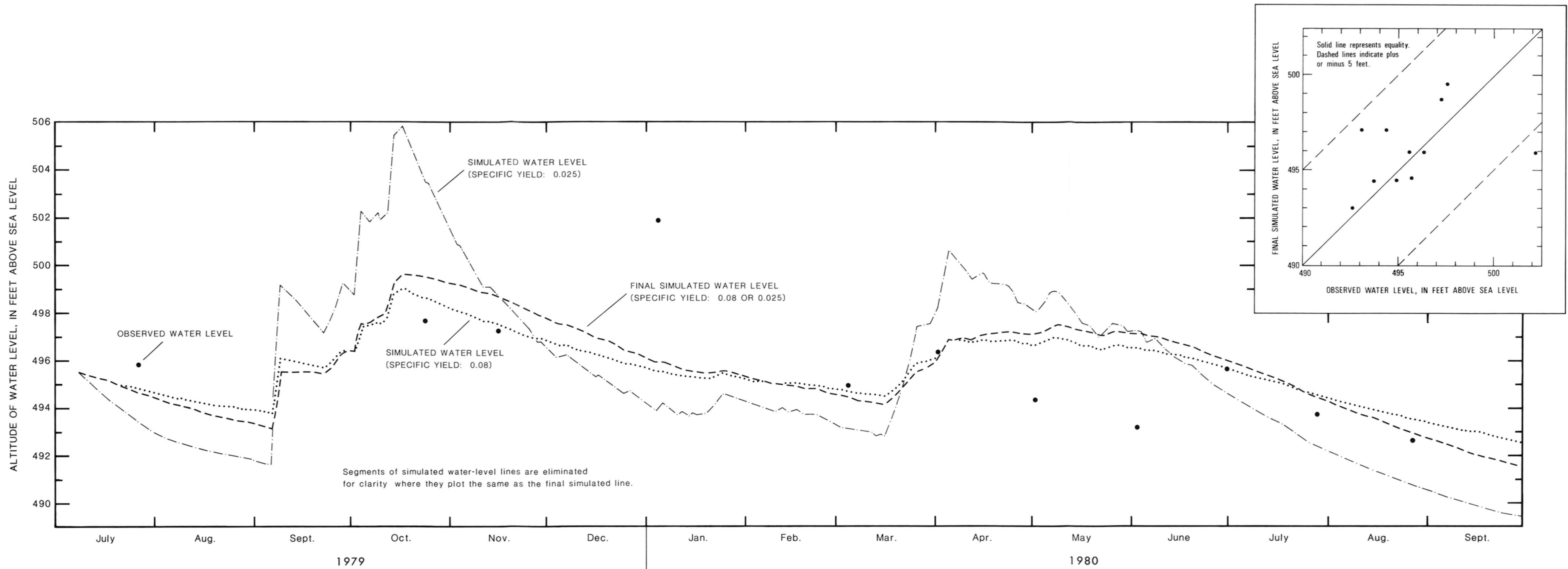
Figure 28. — Simulated water levels, cell C, compared with observed water levels for well HO-BC 38, July 1979 to September 1980.
