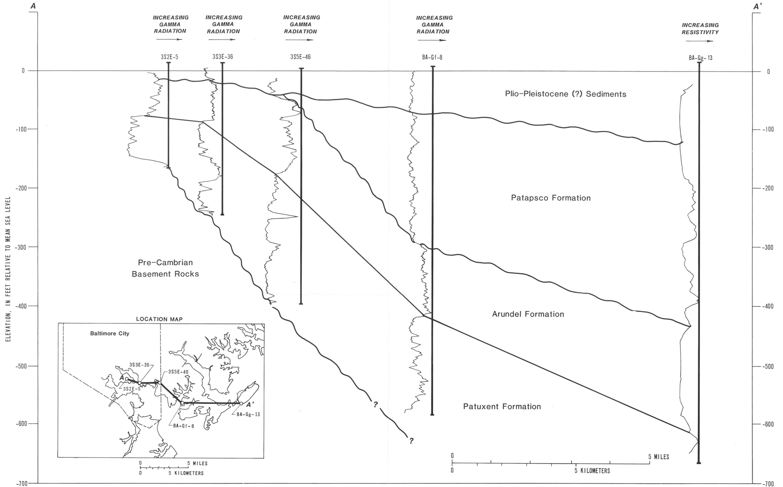
Plate 2.—Cross-section A-A' showing major hydrologic units in the Baltimore, Md., area.
