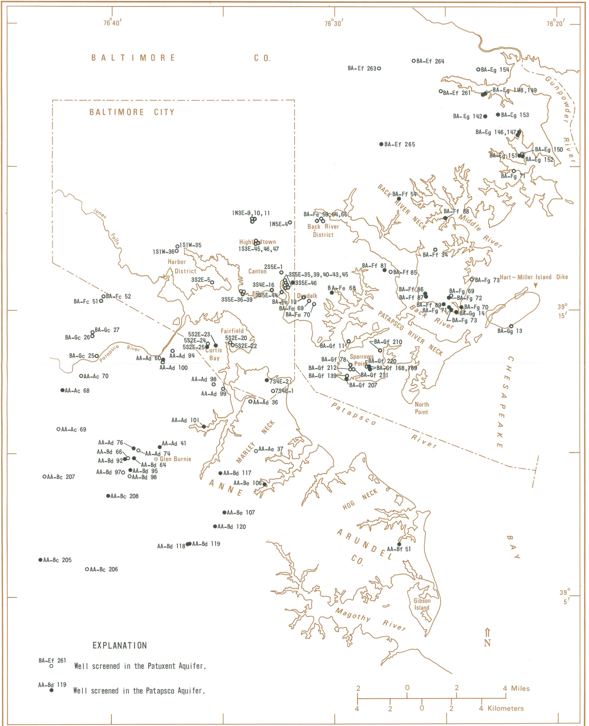
Plate 1.—Locations of Patuxent and Patapsco aquifer wells in the Baltimore, Md., area.
