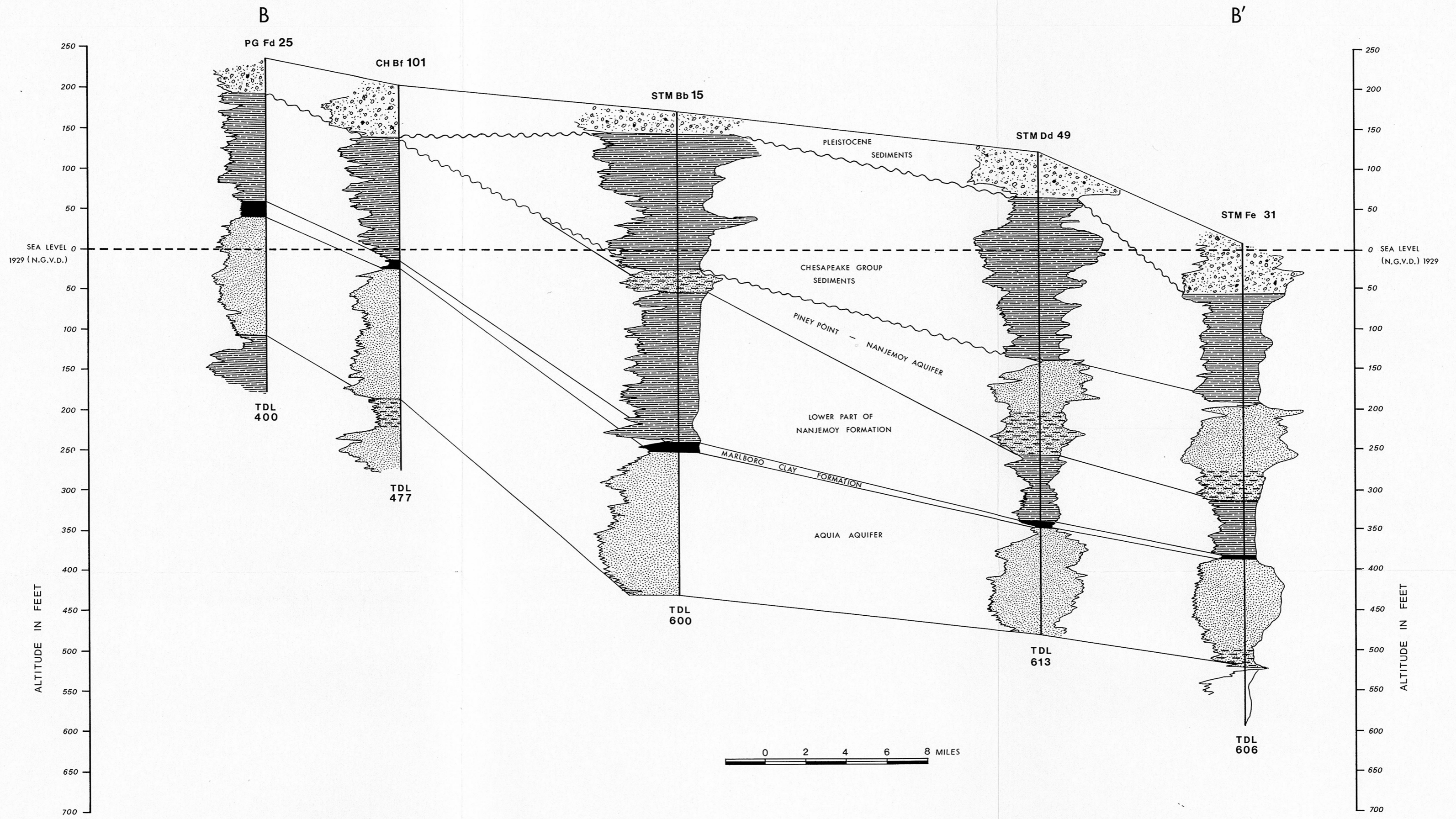
Plate 2.—Cross section B-B' showing major hydrologic units in Southern Maryland
