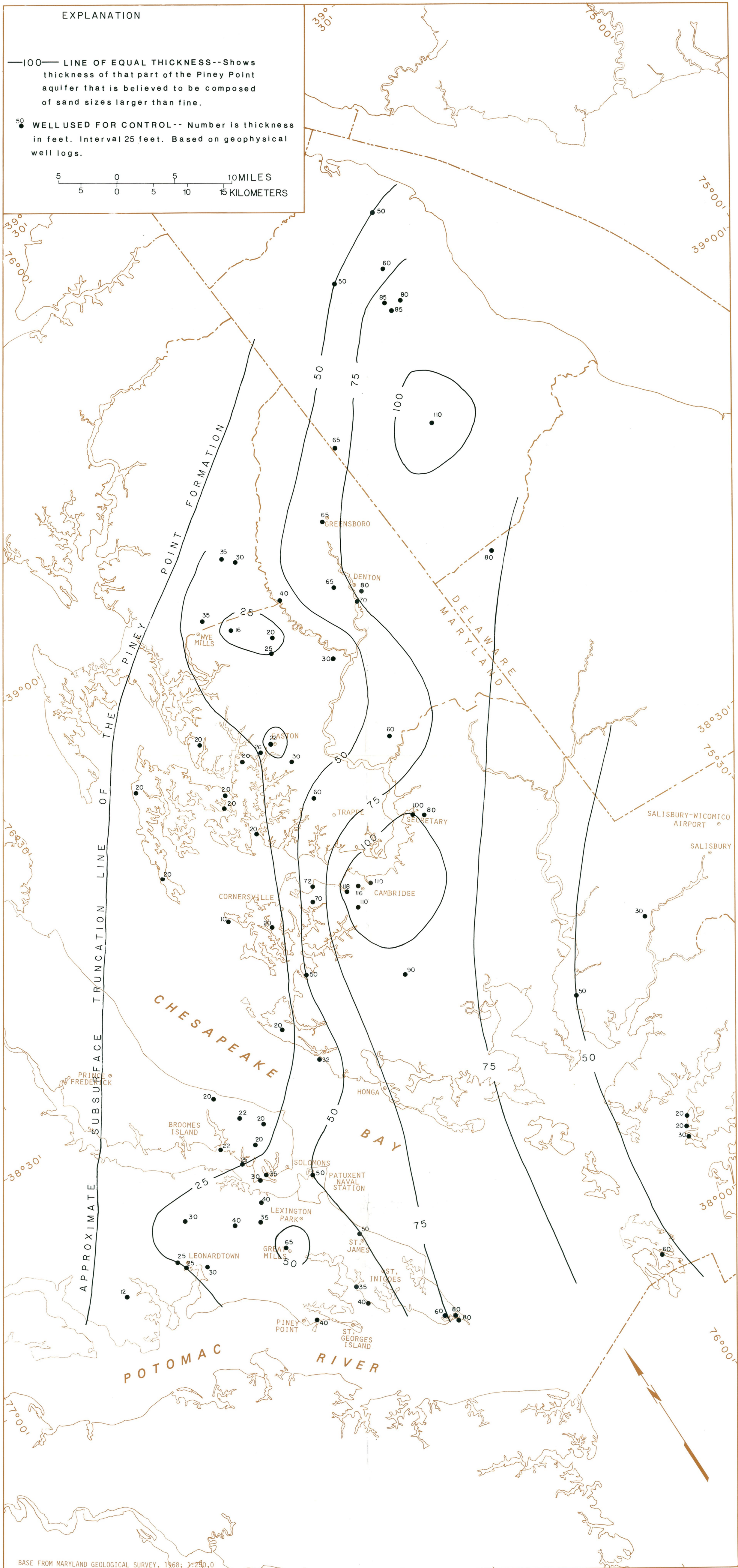
Figure 5.--Effective thickness of the Piney Point aquifer.
